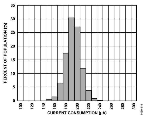
Figure 13. Current Consumption, Measurement Mode, Data Rate = 100 Hz, V_S = V_{DD I/O} = 3.3\text{ V} , 25^\circ\text{C}
