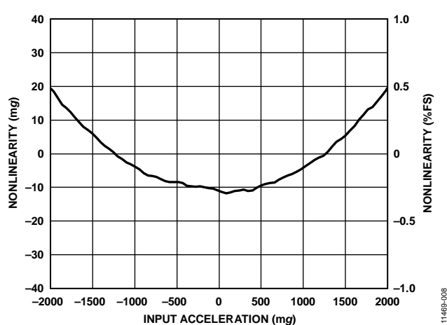
Figure 8. Z-Axis Nonlinearity, ±2 g Input Range
