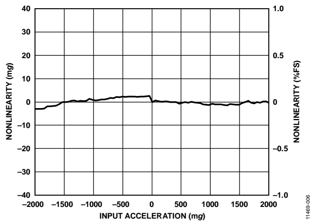
Figure 6. X-Axis Nonlinearity, ±2 g Input Range
